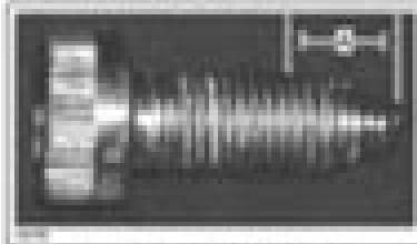
1. Apply oil to the bolts (a). 15 to 16 mm (3/8 in.).
