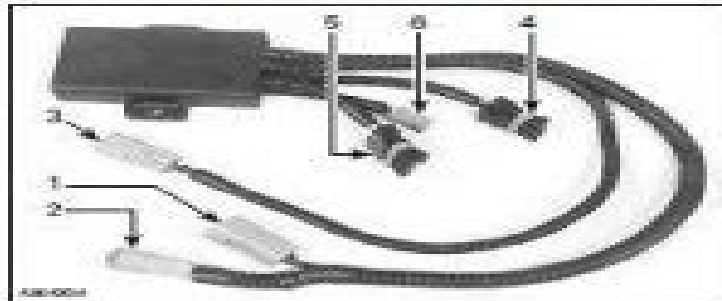
TYPICAL — BOMBARDIER 290 W MPEM — NON-REV MODELS 1. High tension coils, 4-DC housing 2. Generating coils (low and high speed), 4-DC housing 3. Trigger coil, 4-DC housing 4. DESS switch, 4-DC housing 5. DESS pre-amp and ignition coil switch, 4-DC housing 6. External power supply, 4-DC housing
