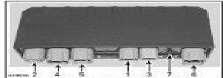
TYPICAL — BOMBARDIER 290 W MPEM — REV MODELS 1. High tension coils, 4-DC housing 2. Generating coils (low and high speed) and trigger coil, 4-DC housing 3. Air temperature sensor, 4-DC housing 4. Trigger coils, 4-DC housing 5. DESS pre-amp, 4-DC housing 6. Reverse switch and alarm, DESS pre-amp and ignition coil switch, 4-DC housing 7. Atmospheric pressure input
