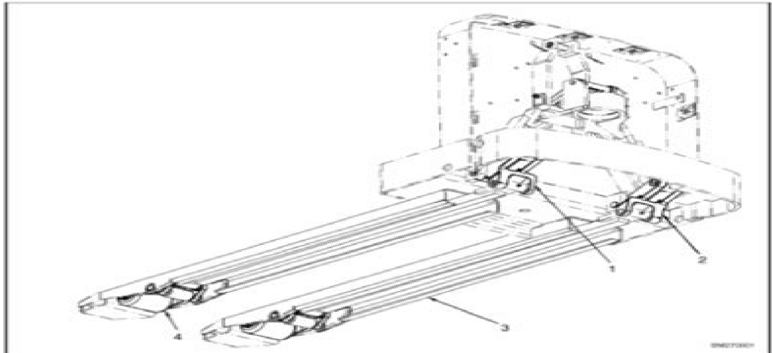
Figure 1. Lift Linkage
