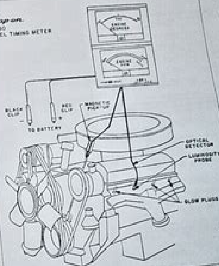
Figure 1 - Typical meter for a 4-cyl with 3.5" offset probe holder
