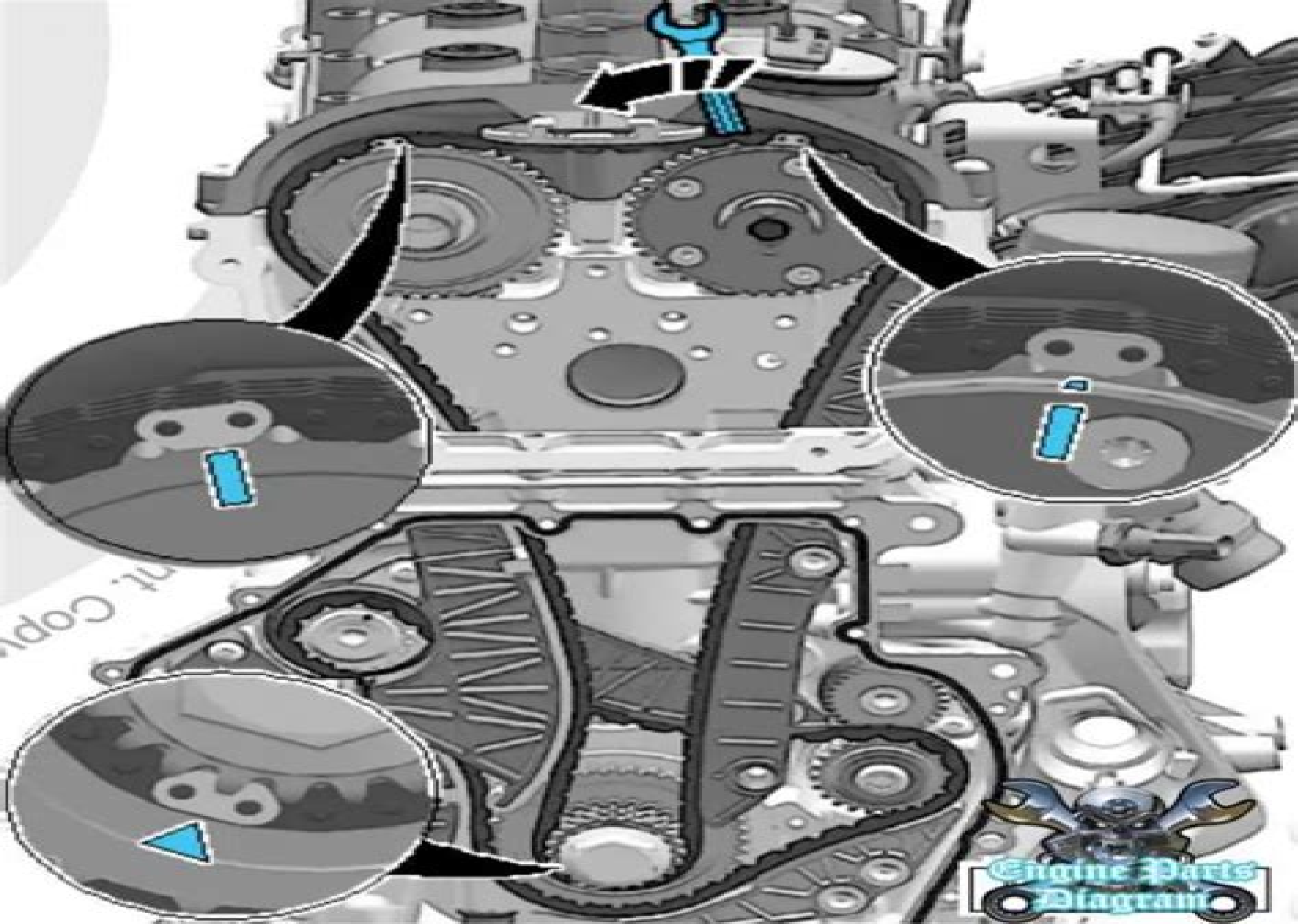
VOLKSWAGEN 2.0 L DIRECT INJECTION ENGINE TIMING MARKS
