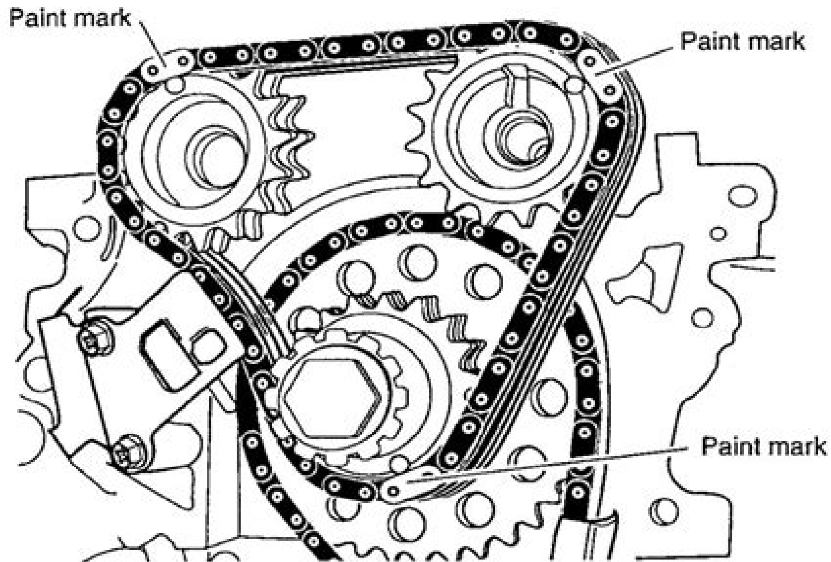
Fig. 14: Outer (Upper) Timing Chain Mating Marks Courtesy of NISSAN MOTOR CO., U.S.A.
