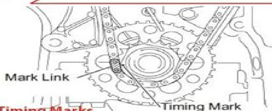
Crankshaft Timing Marks
