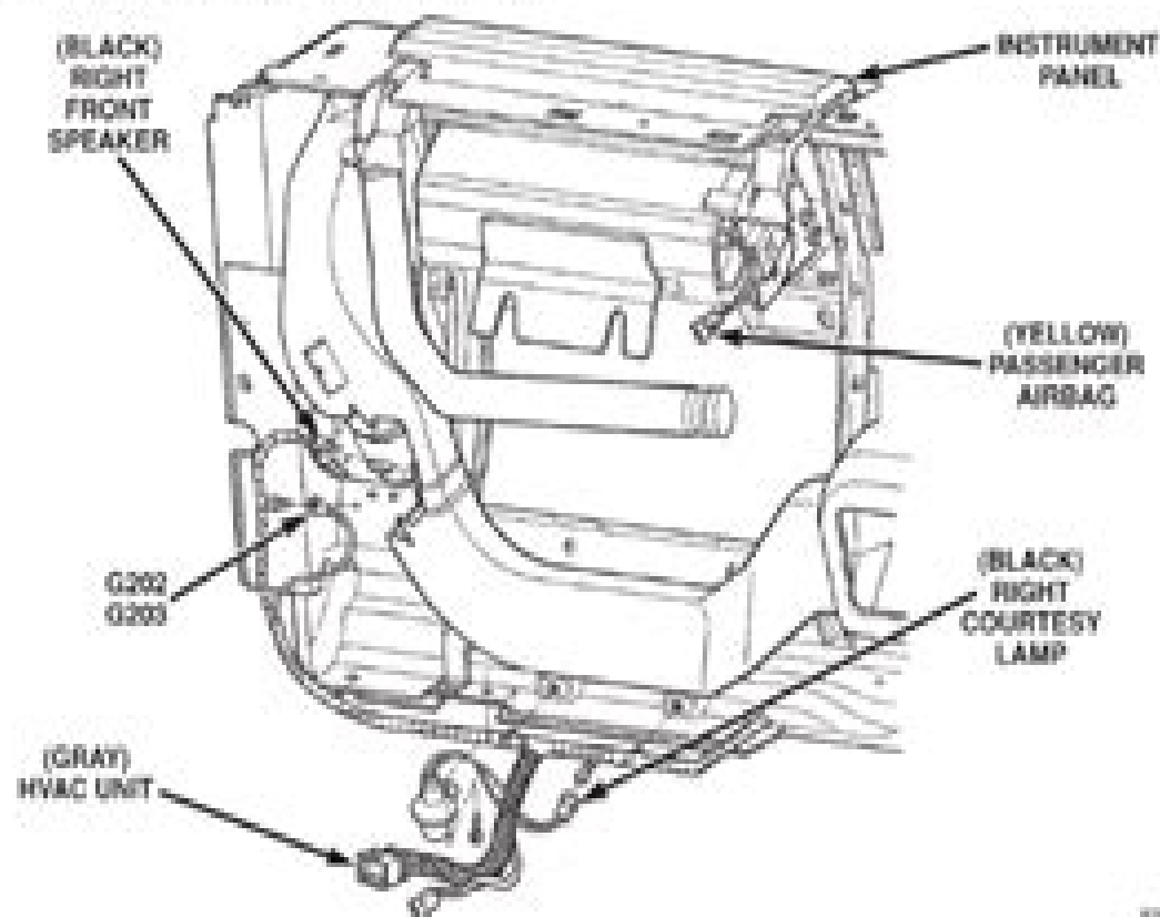
Fig. 21 Instrument Panel Connectors—Right Side, LHD
