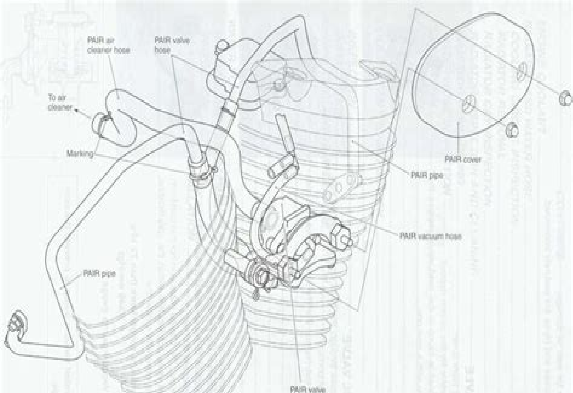
PAIR (AIR SUPPLY) SYSTEM HOSE ROUTING
