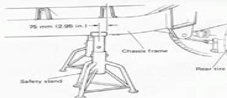
Fig. 0-6 Rear Side
