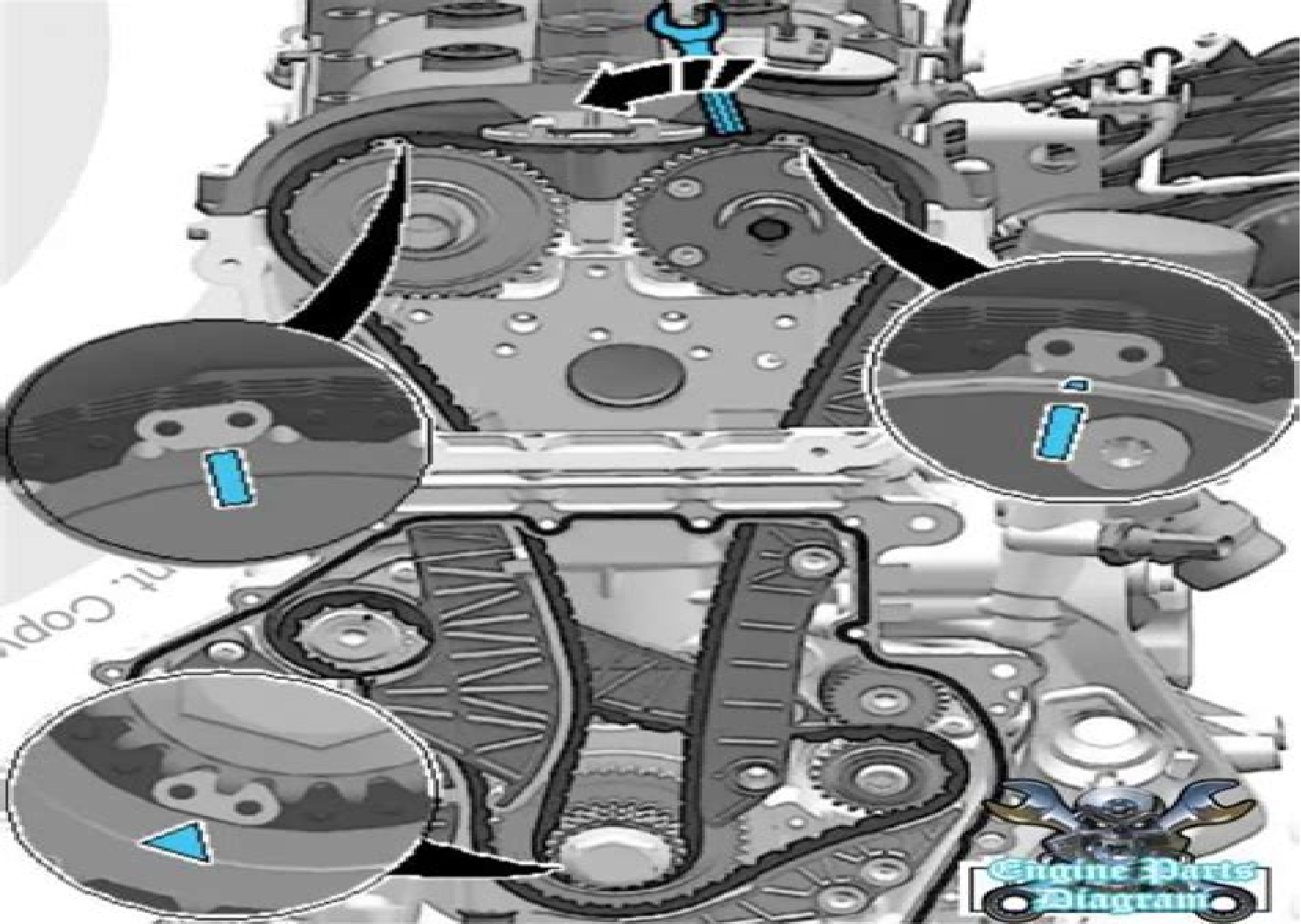
VOLKSWAGEN 2.0 L DIRECT INJECTION ENGINE TIMING MARKS
