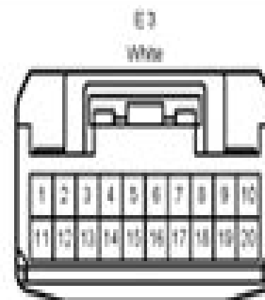
2009 Highlander JBL (non-nav) vs. Joying JBL Harnesses
