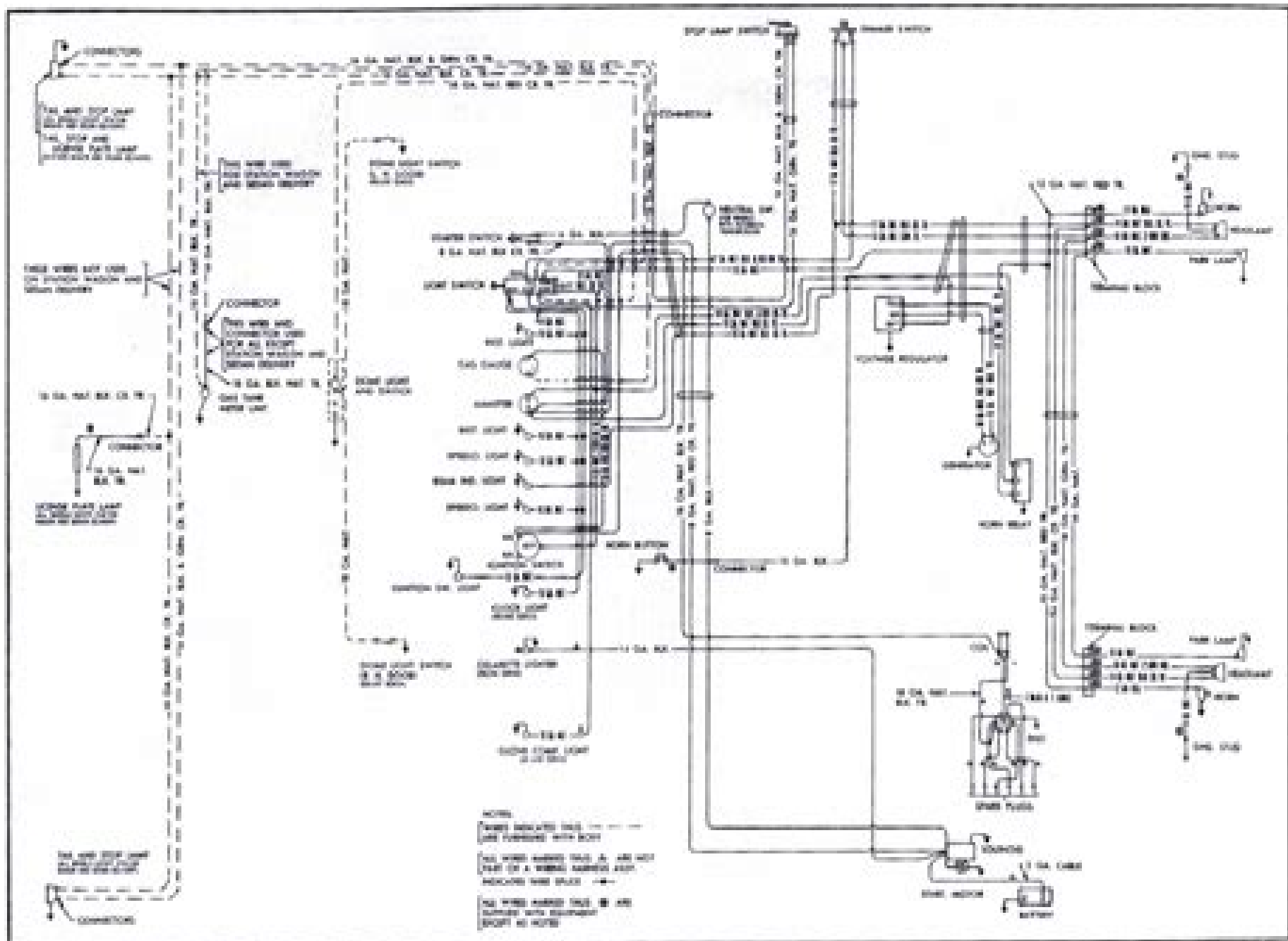
Fig. 3-1951 Passenger Car Wiring Diagram
