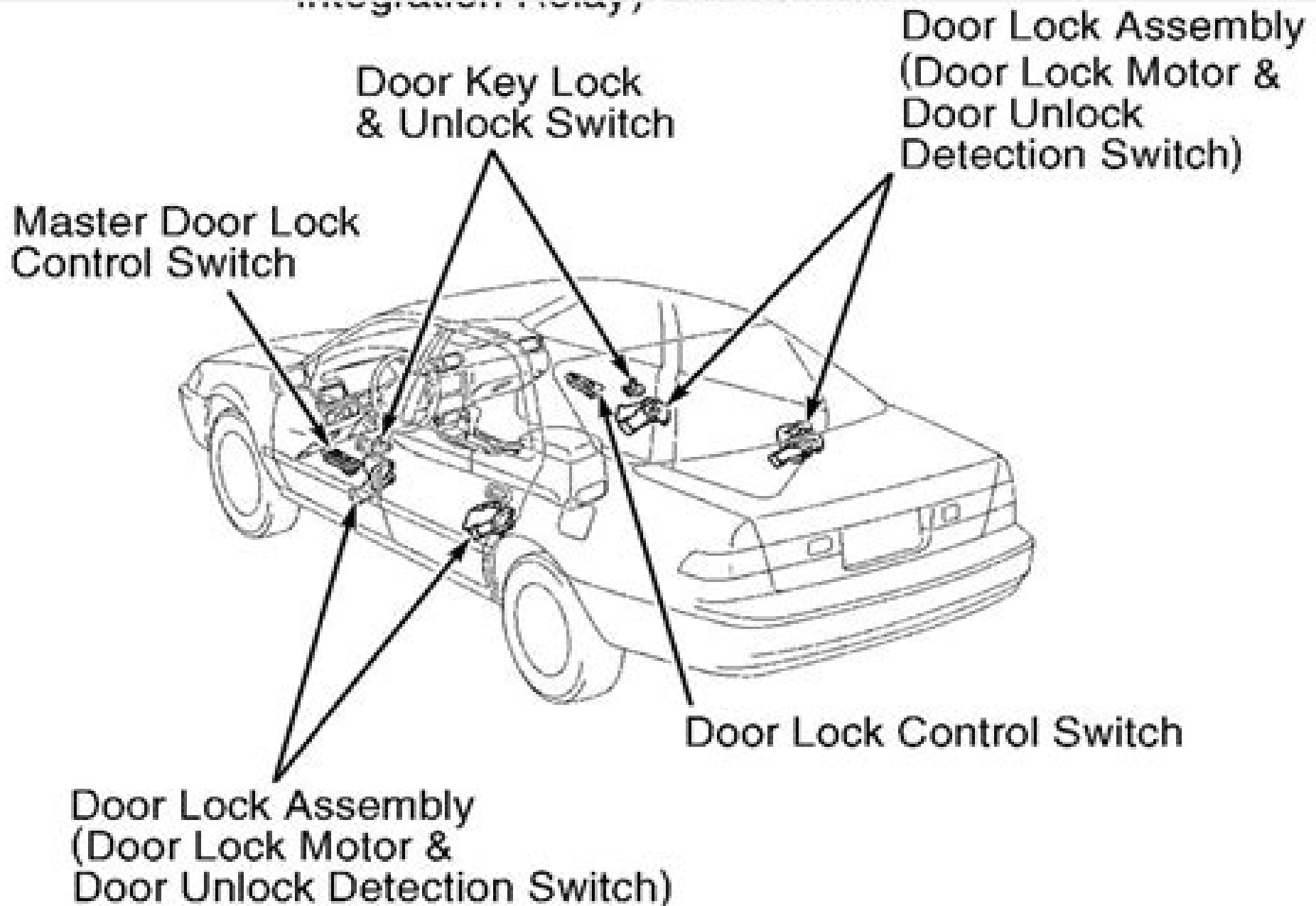
Fig. 2: Locating Power Door Lock Components (Camry)
