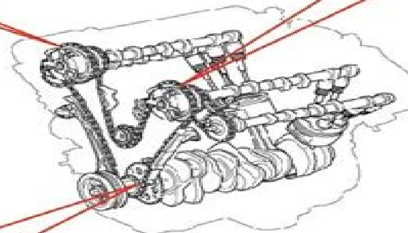
Timing Marks
