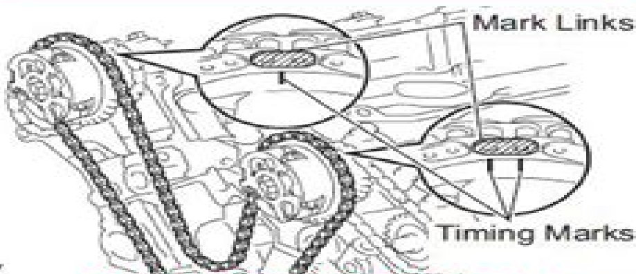
Camshaft Timing Gears Marks
