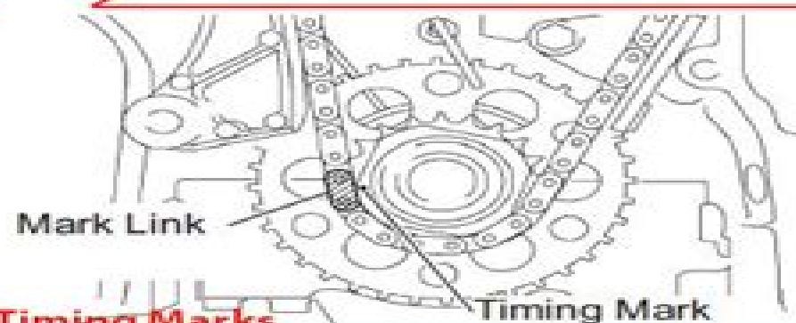
Crankshaft Timing Marks
