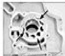
17.4 Note that the valve is with the painted dots (crankshaft facing the oil pump cover) - 1.4 litre engine
