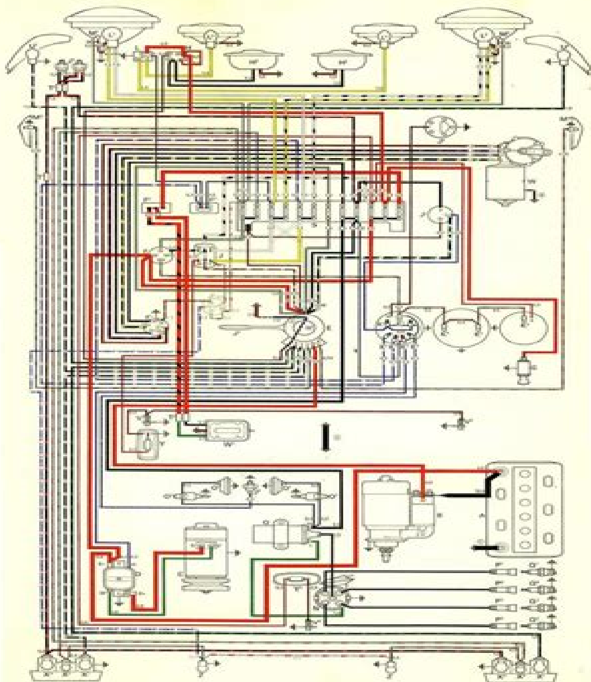
Wiring Diagram VW Karmann-Ghia-Models (from August 1966, Chassis No. 347-000-001)
