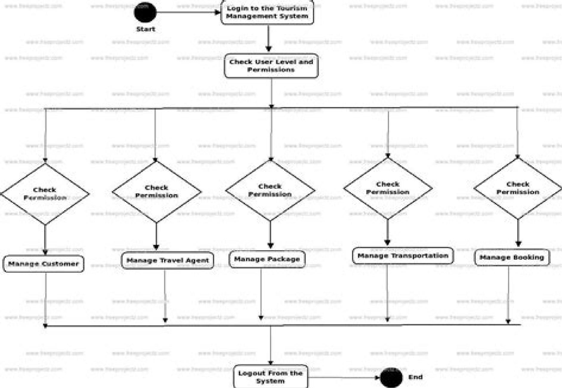
Activity Diagram for Tourism Management System
