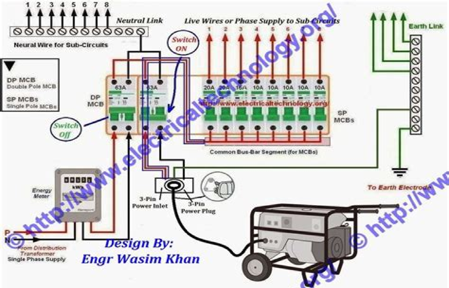
Generator Connection Diagram to Home Supply System In case of, when Power supply is not available from Power House (In this Case, Generator Supply Electricity to Home Appliances)
