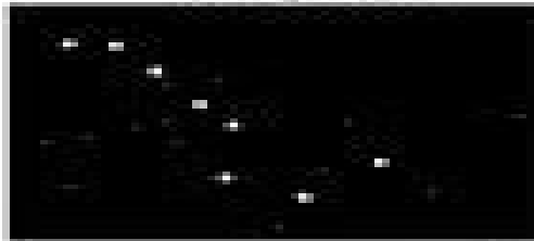
12. Big Dipper
