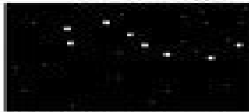
13. Little Dipper
