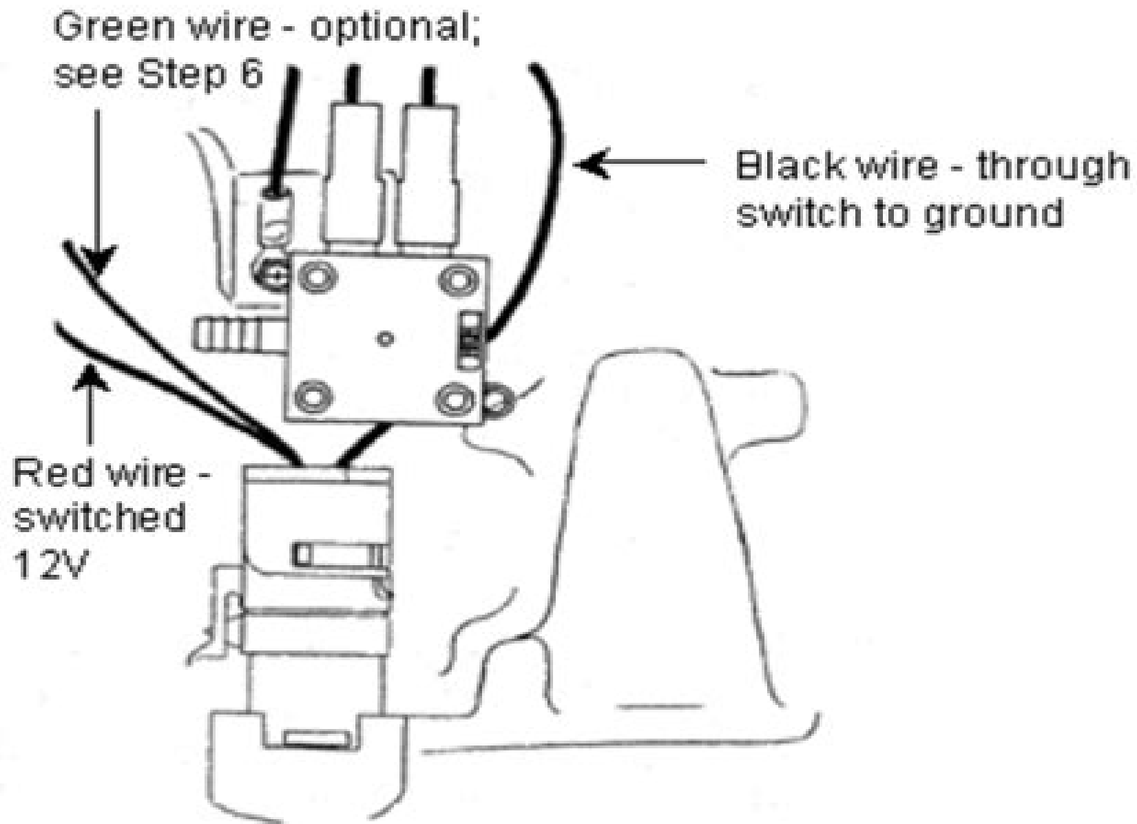
Figure 4 - External Wiring Configuration
