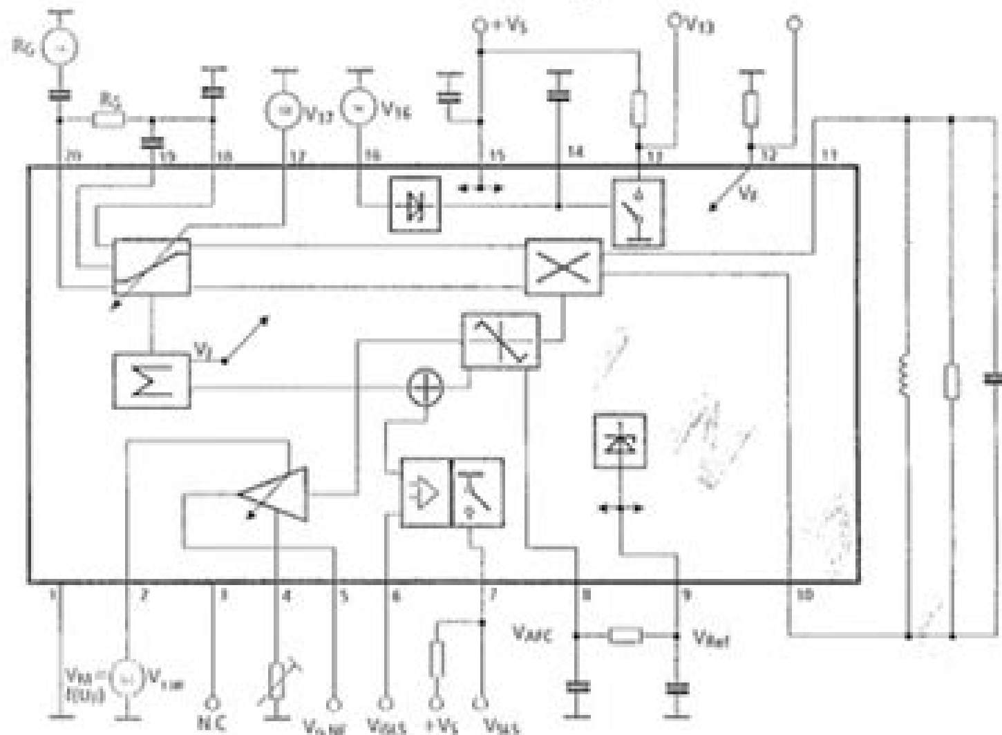
Block Diagram
