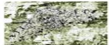
3. Light gray peppered moth on the light gray colored tree
