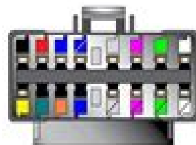
Sony - 16 Pin
