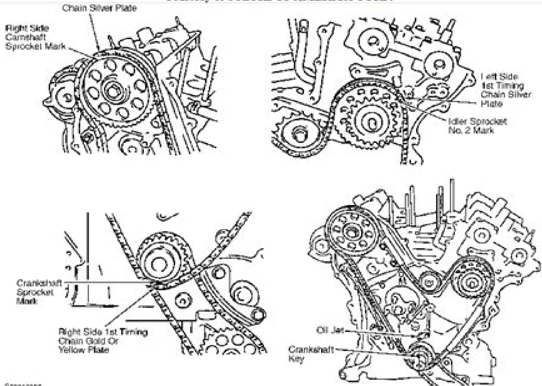
Fig. 11: Aligning Marks On Right 1st Timing Chain
