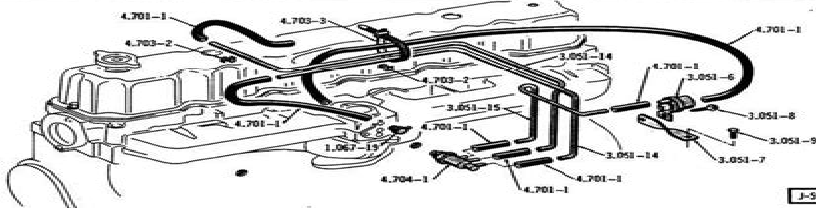
VACUUM ADVANCE MODULATION SYSTEM . . . 80 (SIX-CALIF)
