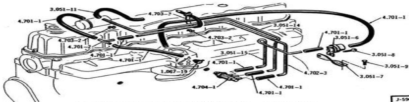
VACUUM ADVANCE MODULATION SYSTEM . . . 10-20-40 (SIX)
