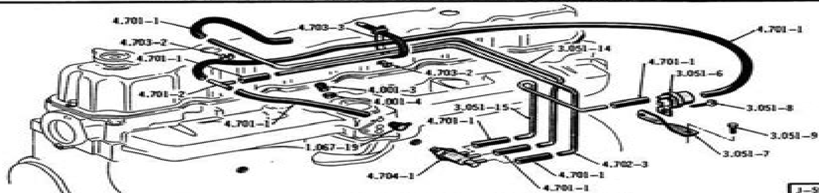
VACUUM ADVANCE MODULATION SYSTEM . . . 80 (SIX-E/ CALIF)
