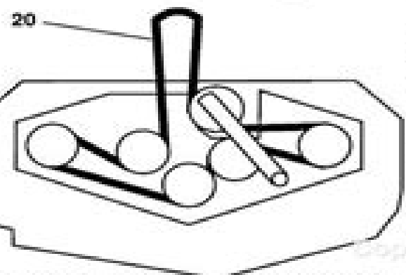
52" Deck Belt Routing
