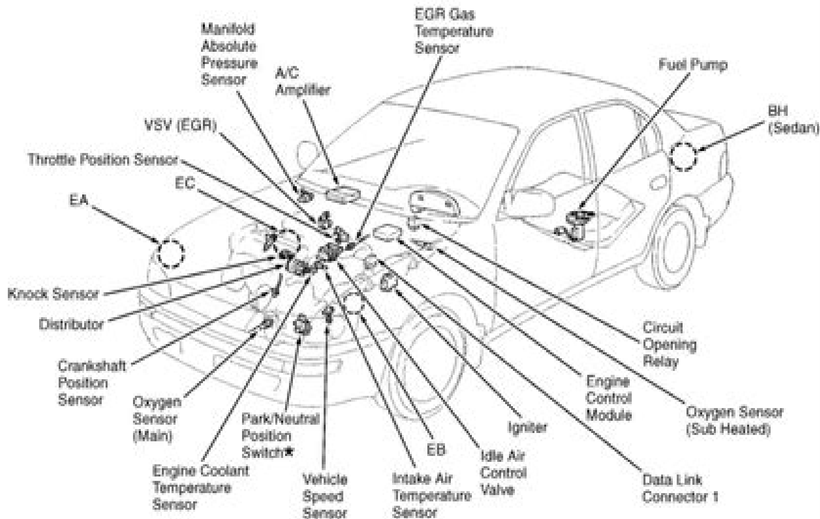
Fig 2. Vehicle Overview (1.8L)
