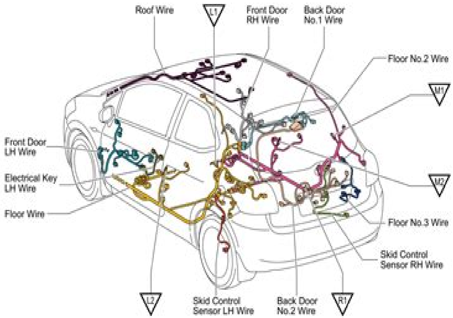
Ground Points in Body -LHD 3-Door W/B
