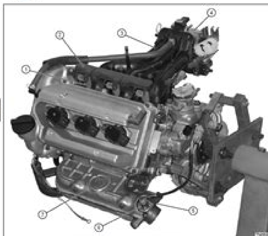
1 Injector (each) 2 Fuel Rail 3 Intake Manifold 4 Throttle Body Assembly 5 Exhaust Manifold 6 Oxygen Sensor 7 Heat Shield
