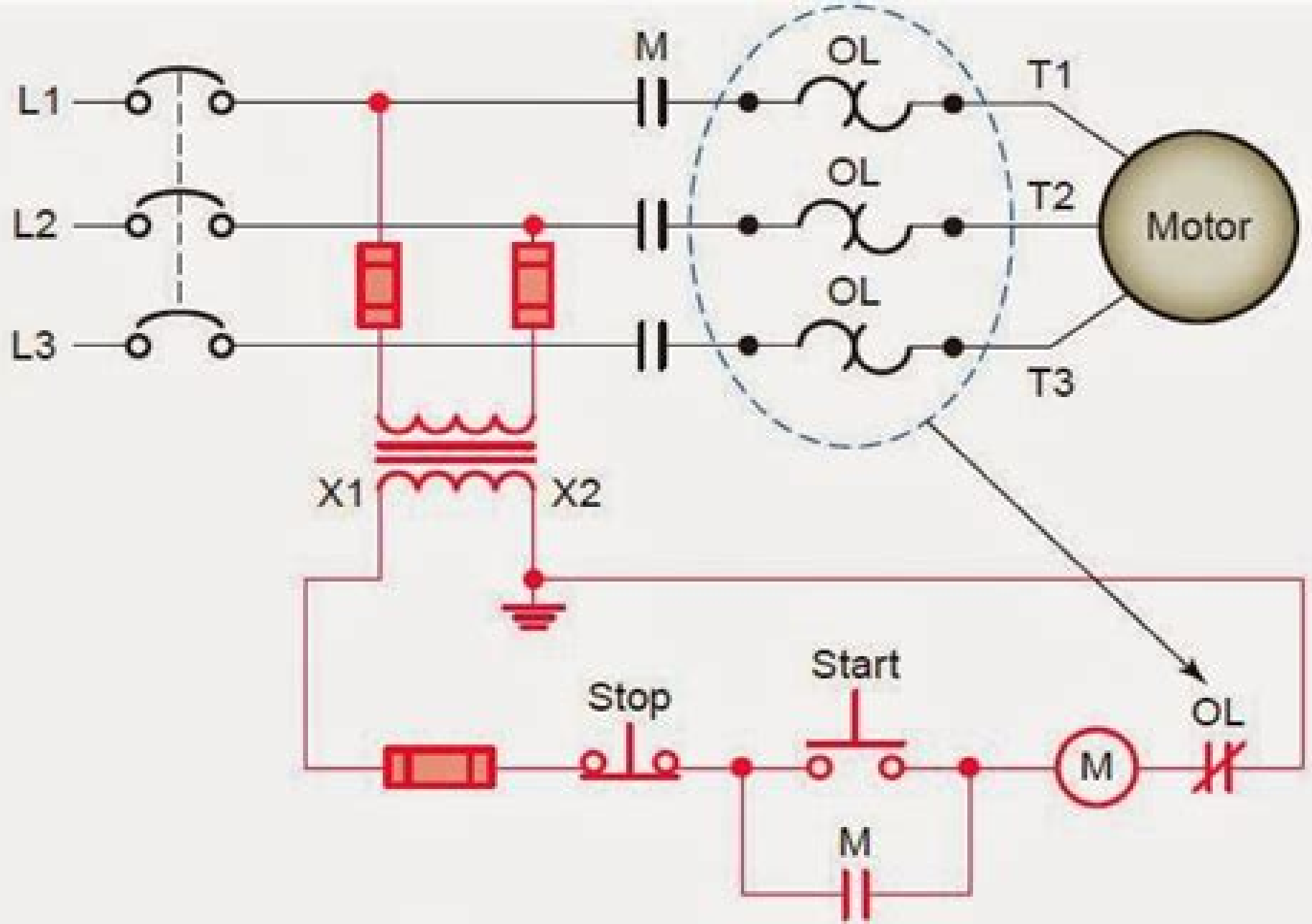
Thermal overload relay circuit operation
