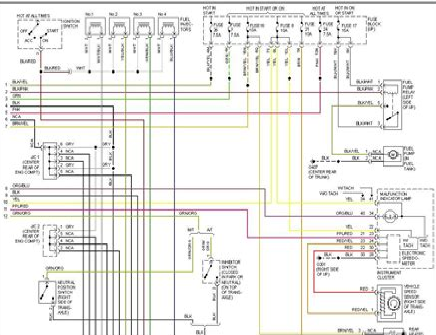
1995 Nissan Sentra GXE-Fig. 14: 1.6L, Engine Performance Circuits (2 of 2)
