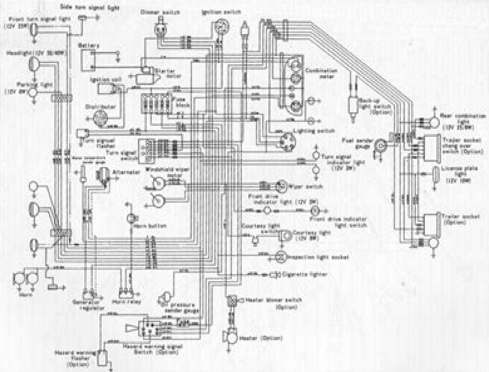
WIRING DIAGRAM (F140(I), 45(I), 45(I)V, 43(I))
