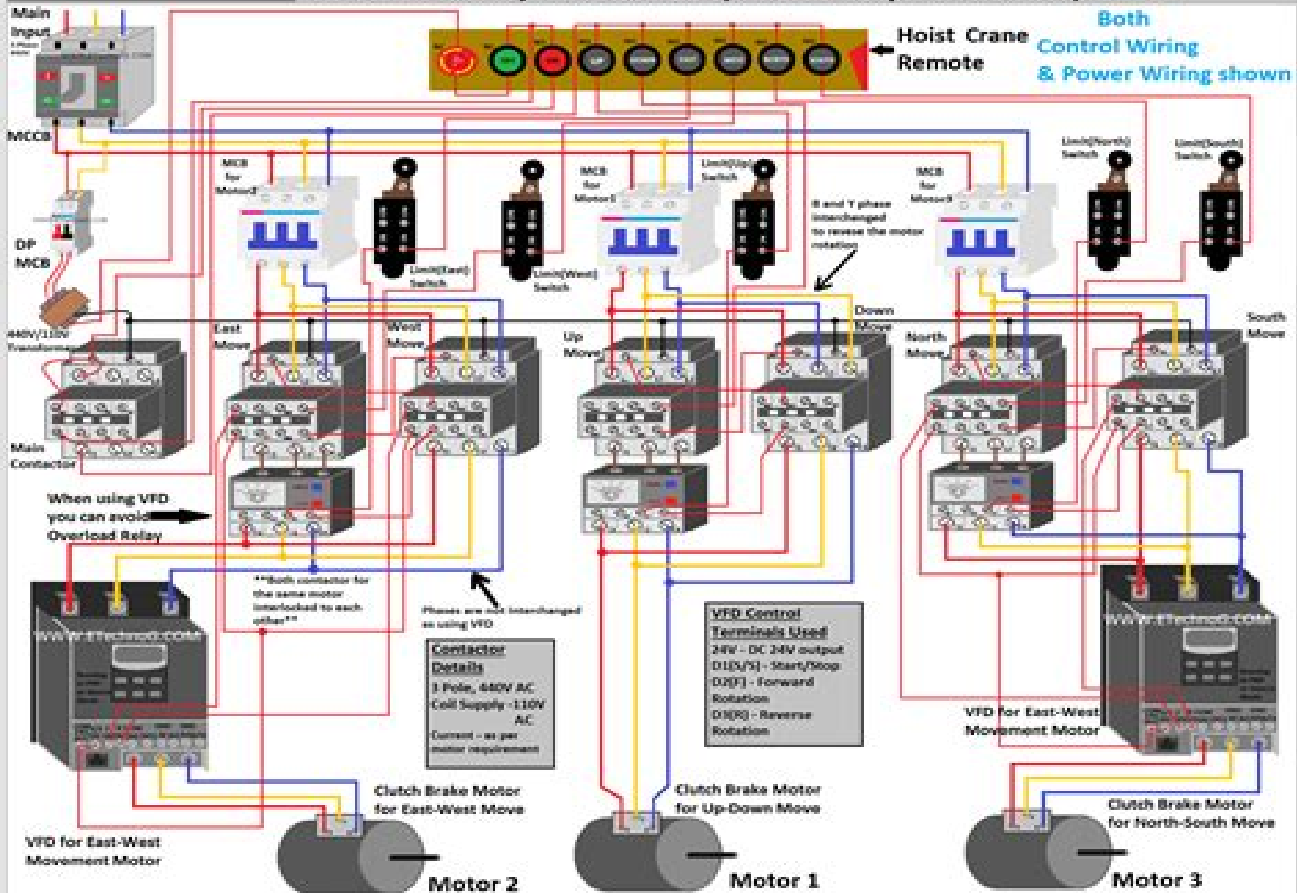
EOT Crane Wiring Diagram and Connection with Motor, Contactor, Remote, Switches, VFD
