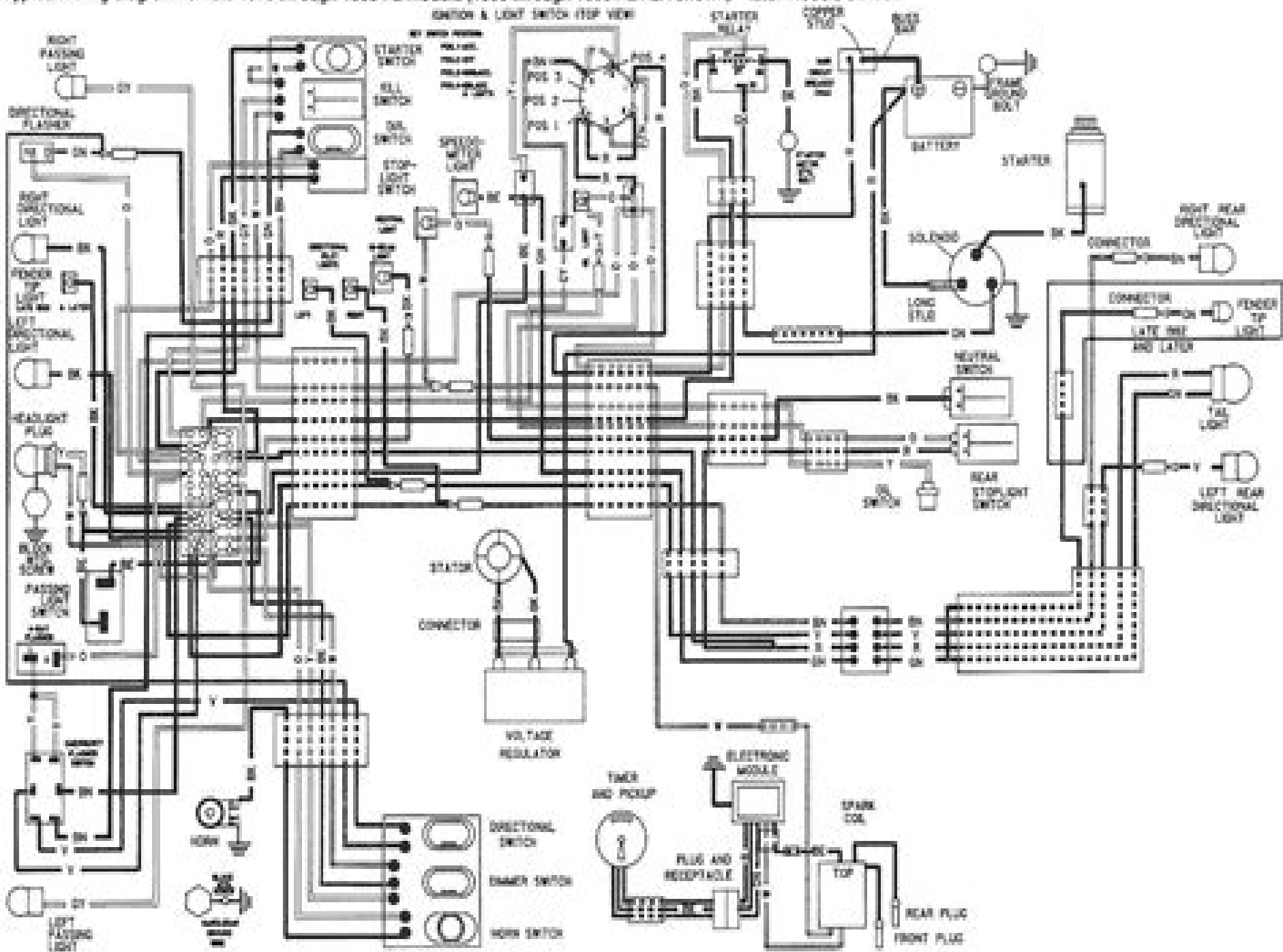
Typical wiring diagram for late 1978 through 1983 FL models (1980 through 1983 FL/FLH shown) - later models similar
