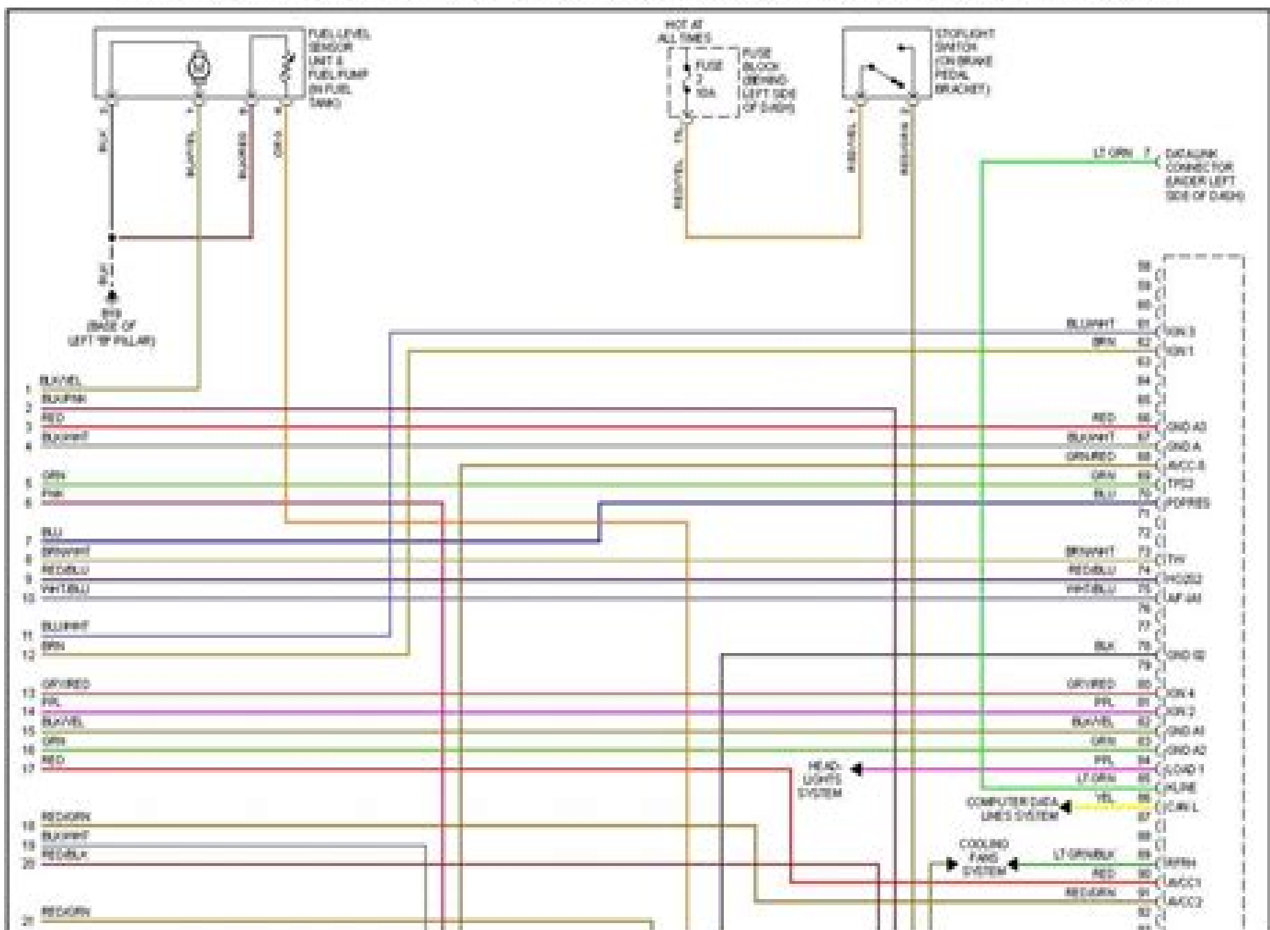
2003 Nissan Sentra GXE-Fig. 19: 1.8L, Engine Performance Circuit, SULEV (4 of 4)
