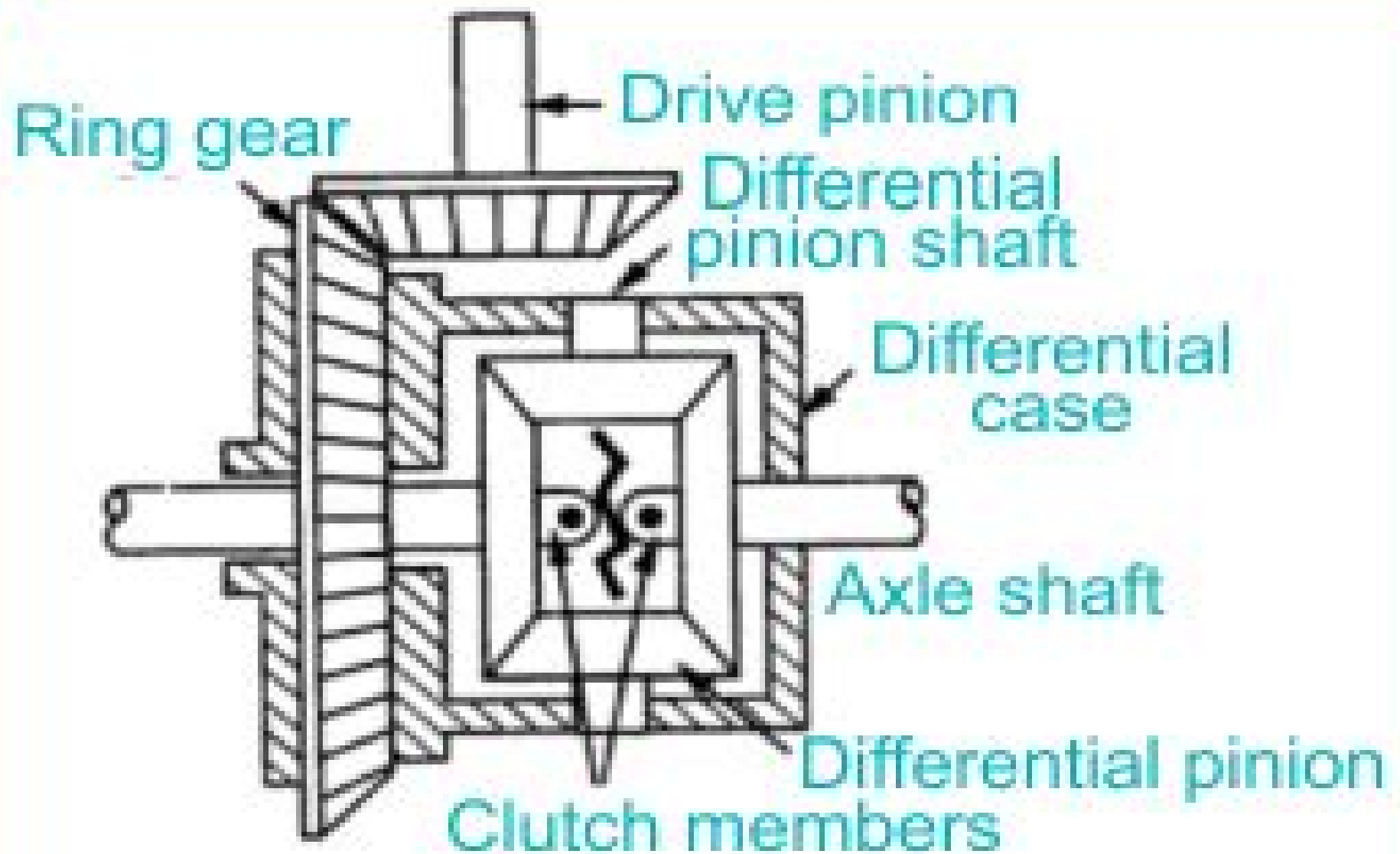
Limited Slip Differential
