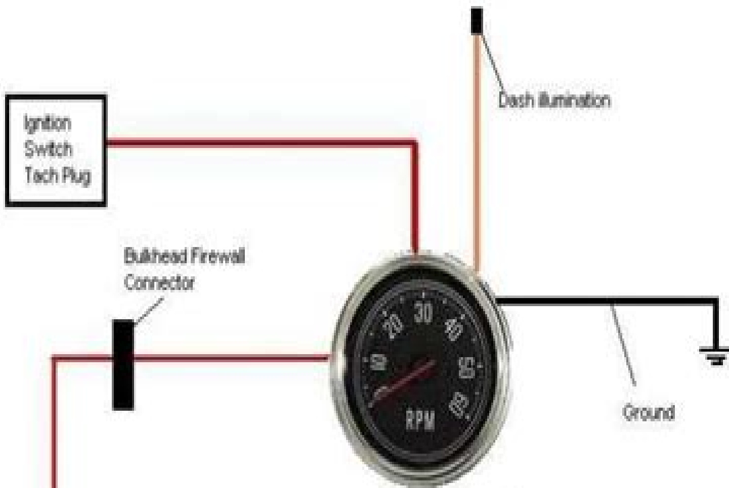
Jeep CJ Tachometer Wiring 1980 - 1986 6 and 8 cylinder
