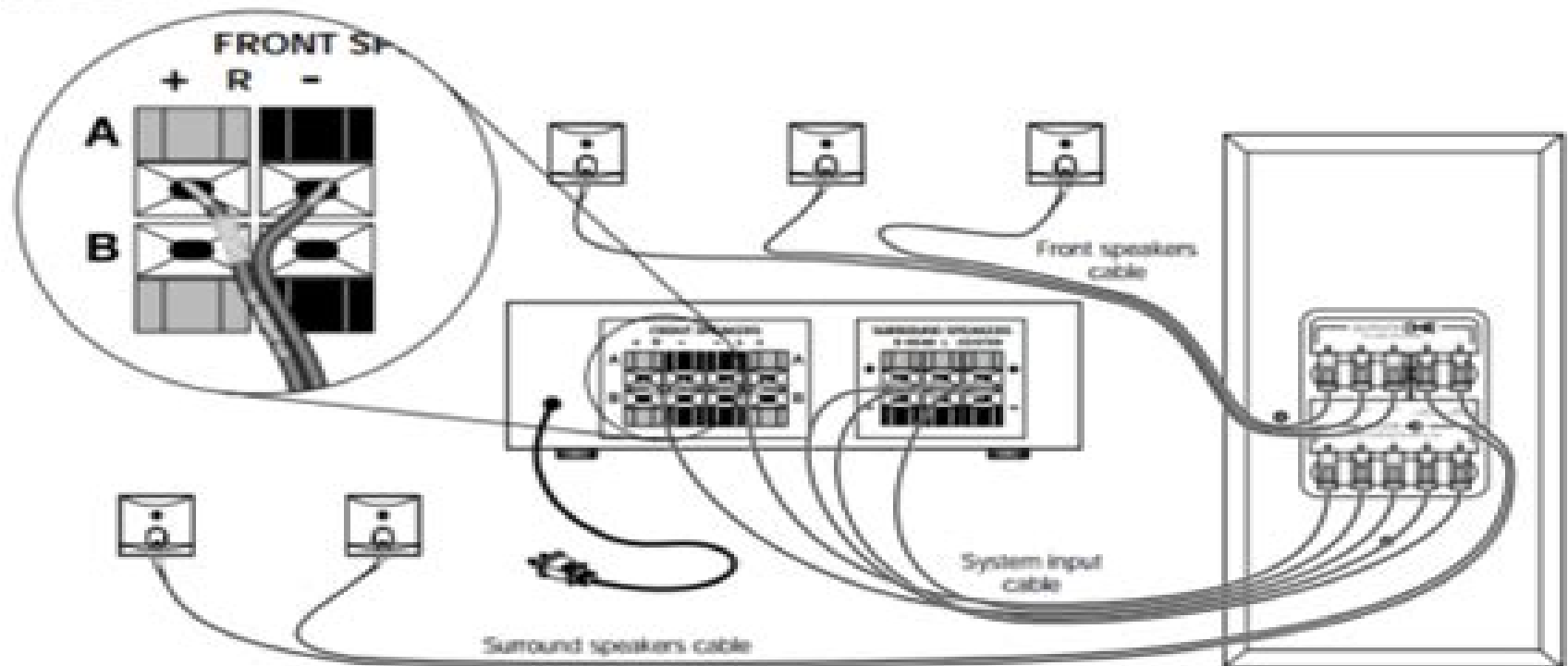
Figure 8 System Connections
