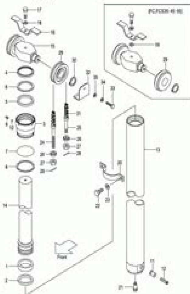
FIG.131 LIFT CYLINDER (FRONT)(FM81M) (OPTIONAL) (HYD.)
