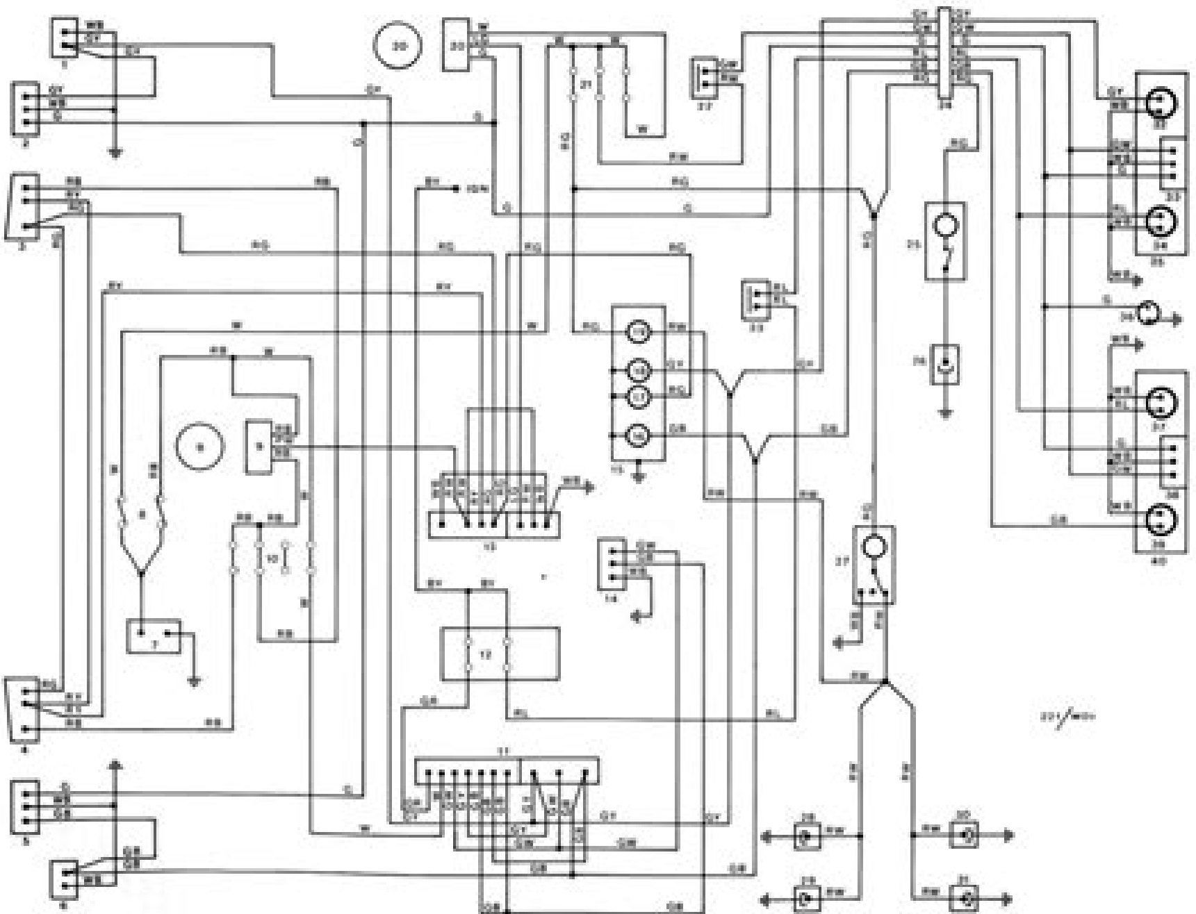
Wiring diagram of lamp circuits
