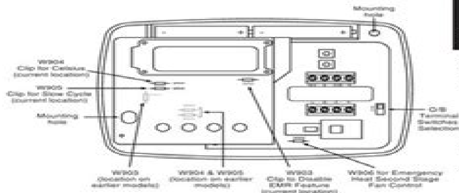
Figure 1. Thermostat base
