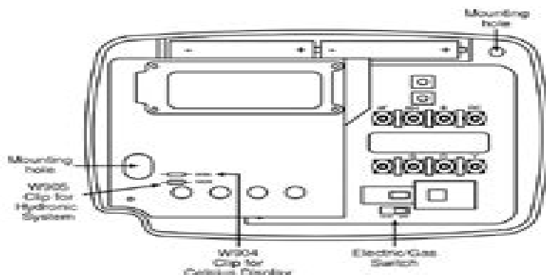
Figure 1. Thermostat base
