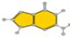
Nucleobases
