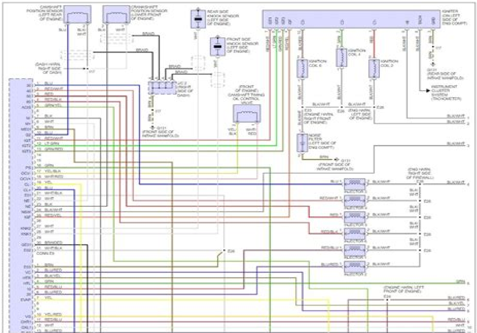
Fig 1: 3.0L Non-Turbo, Engine Performance Circuits (1 of 4)
