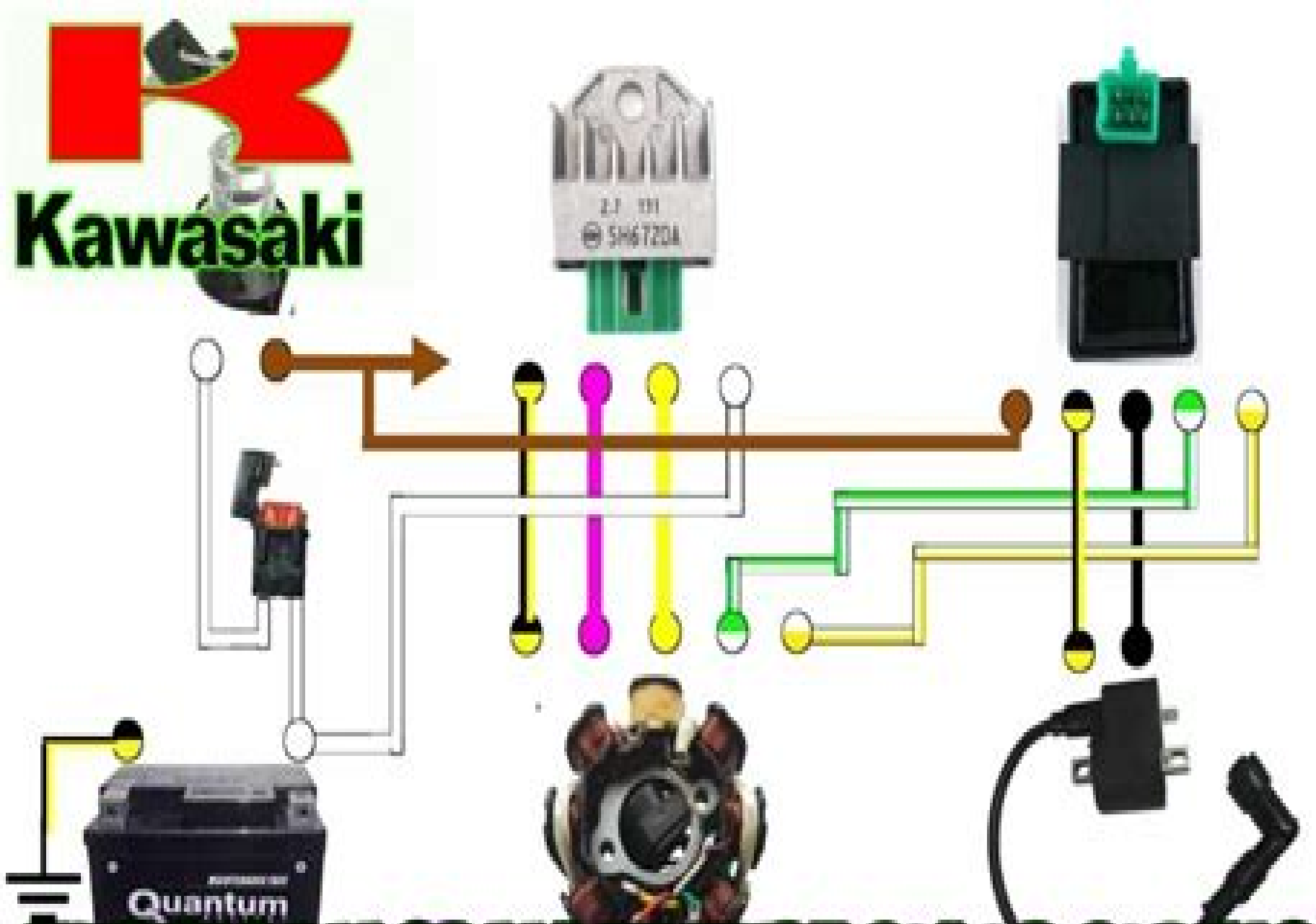
WIRING DIAGRAM AT WIRE COLOR CODING
