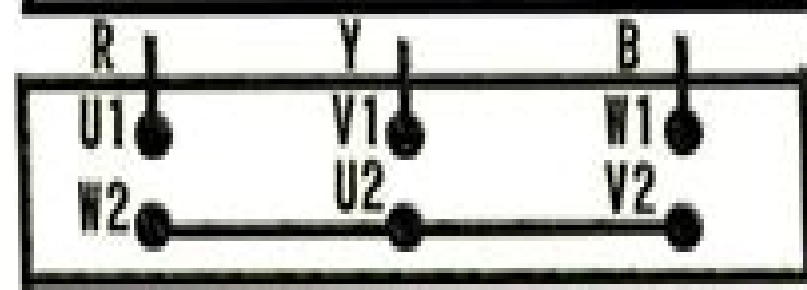
MOTOR TERMINAL BOX STAR CONNECTION
