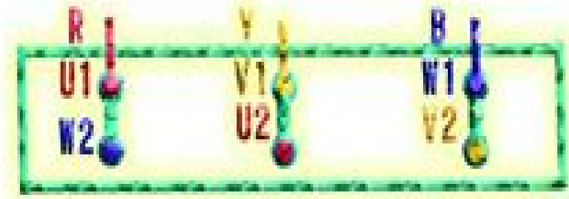
MOTOR TERIMANAL BOX DELTA CONNECTION
