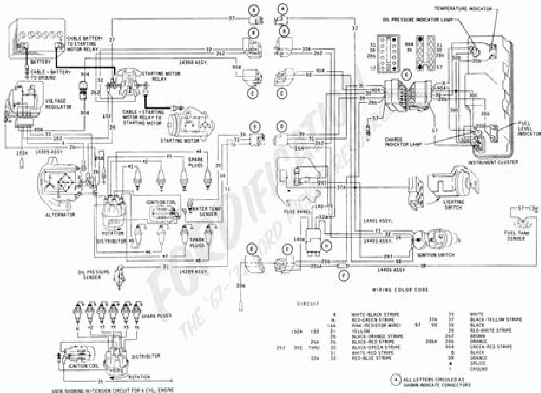
1967 F-100 THRU 350 SERIES TRUCK IGNITION, CHARGING, STARTING AND GAUGES
