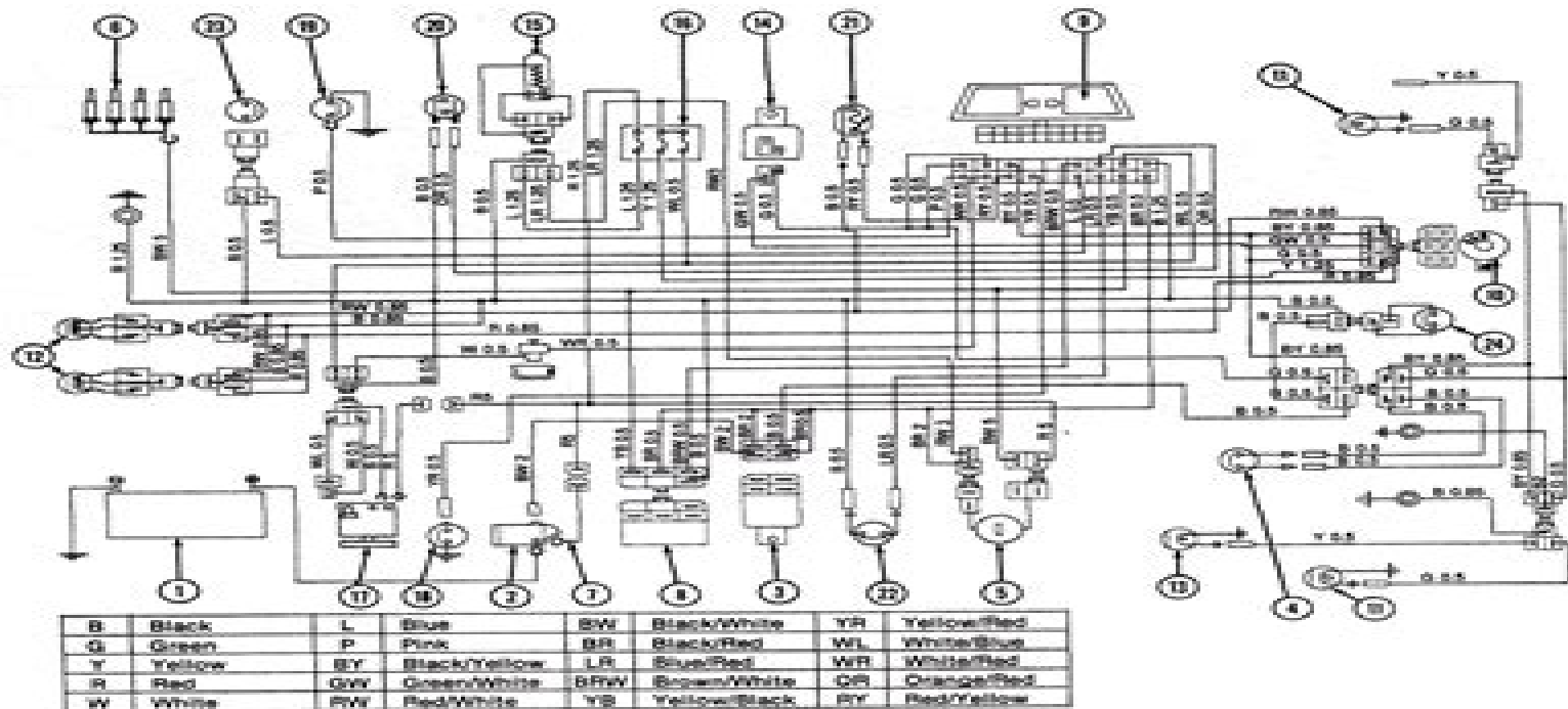
Figure 2 Wiring Diagram — Model 2120 1. Battery 15. Engine Stop Solenoid 2. Starter Motor 16. Fuse Box 3. Neutral Start Relay 17. Alternator Assy. 4. Neutral Start Switch 18. Temperature Sender Unit 5. Key Start Switch 19. Oil Pressure Sender Unit 6. Glow Plugs 20. Air Cleaner Sender Unit 7. Fusible Link 21. Fuel Sender Unit 8. Glow Timer 22. Parking Brake Switch 9. Instrument Warning Lights 23. Reserve Tank Sender Unit 10. Combination Switch (Flasher/Head Lights) 24. Neutral Start Switch — Main Change Lever 11. Flasher Warning Lights 12. Head Lights 13. Tail Light 14. Flasher Unit
